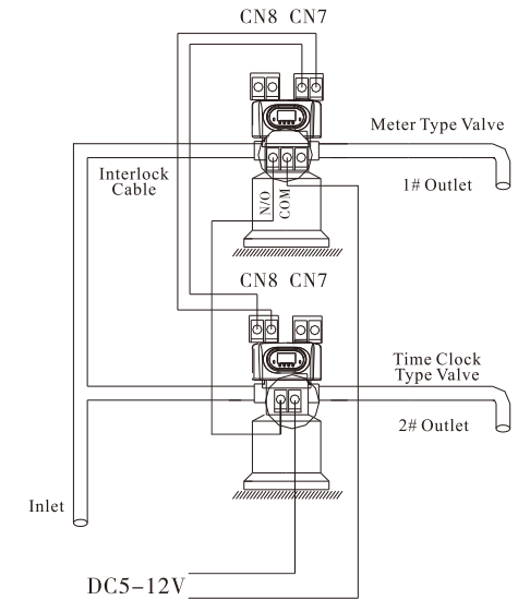
Figure 3-13 Series system
