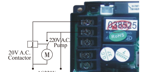
Figure 3-8 Wiring of Booster Pump on Inlet
