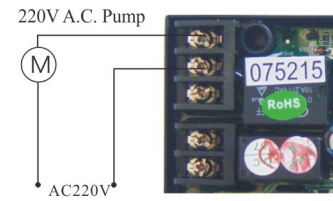
Figure 3-7 Wiring of Booster Pump on Inlet
