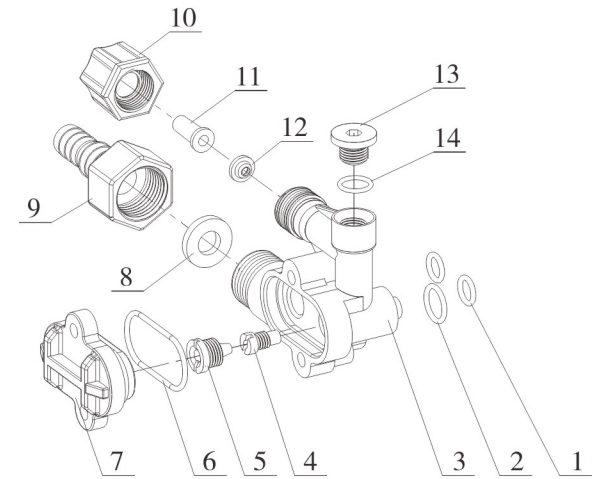
Old Injector (6300 series) Components:
