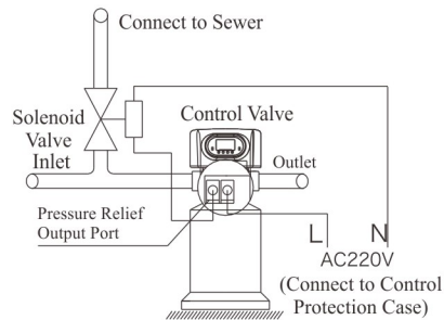
Figure 3-10 Wiring of Pressure Relief Output Connector
