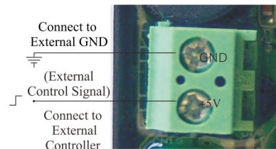
Figure 3-11 Wiring of Remote Handling Connector
