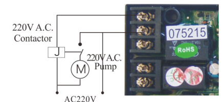
Figure 3-8 Wiring of Booster Pump on Inlet
