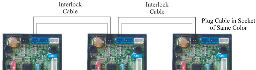
Figure 3-9 Wiring of Interlock Cable
