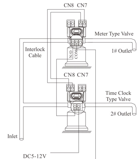
Figure 3-13 Series system
