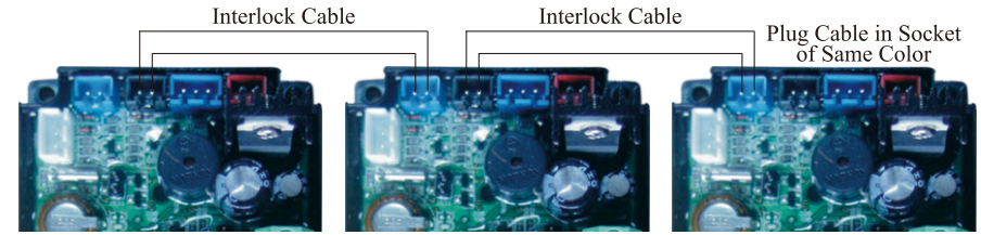
Figure 3-10 Network System Wiring with Interlock Cable
