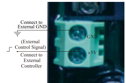
Figure 3-12 Wiring of Remote Handling Connector
