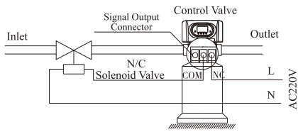
Figure 3-3 Wiring of Solenoid Valve on Inlet
