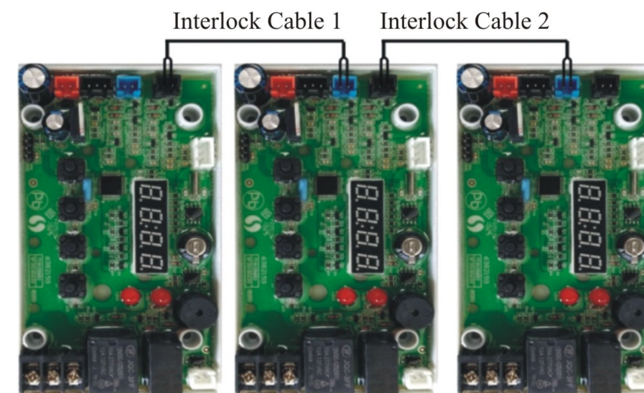
Figure 3-9 Interlock
