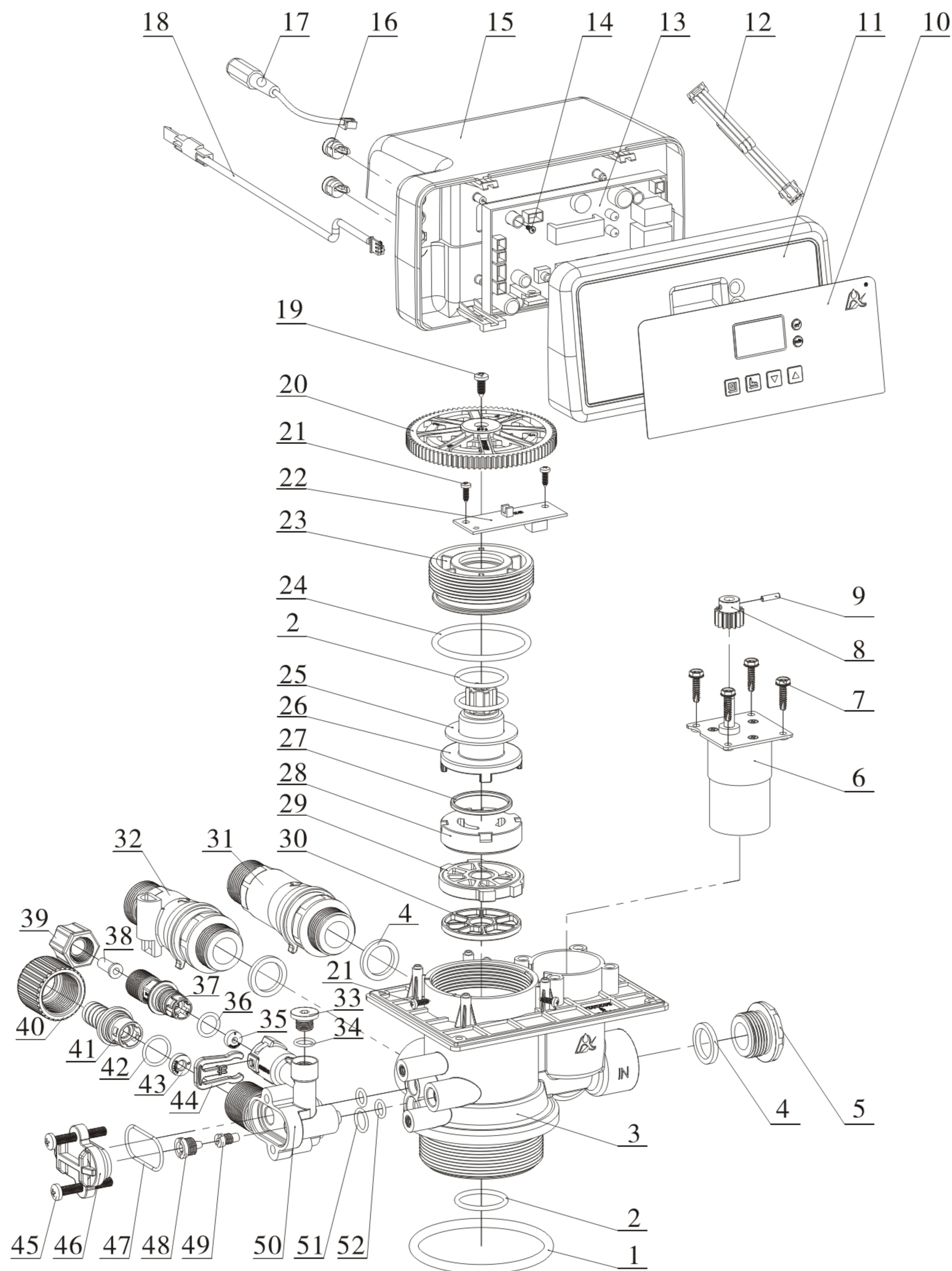
Construction figure of F69Q3:
