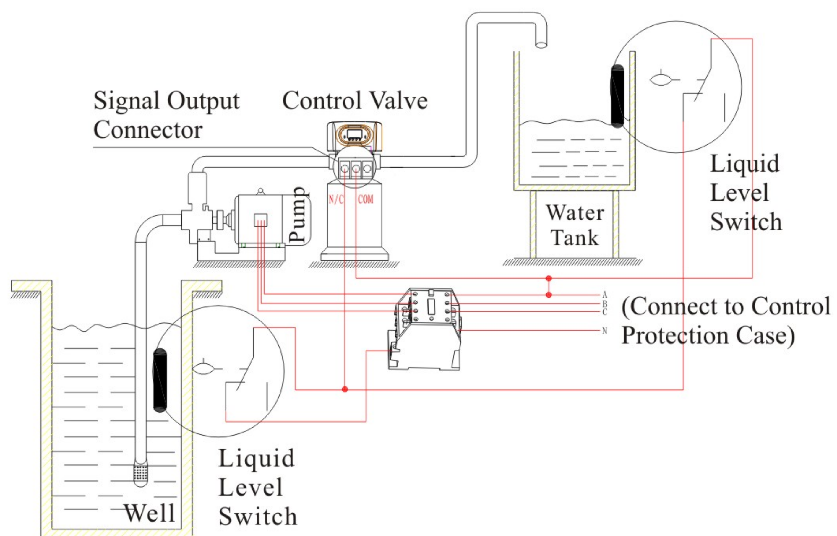
Figure 3-6 Wiring of Liquid Level Switch in Water Tank Controls Inlet Pump 4) Control Inlet Booster Pump (Set as b-01 or as b-02)
