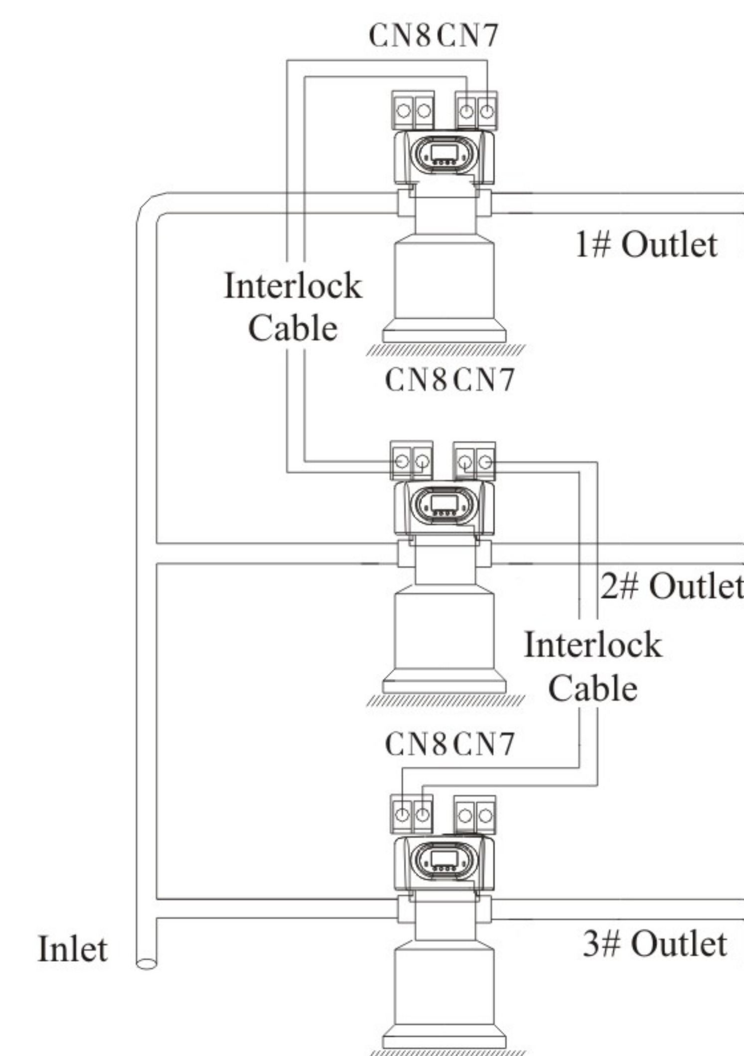
Figure 3-10 Supply Water at Simultaneously and Regenerate Separately
