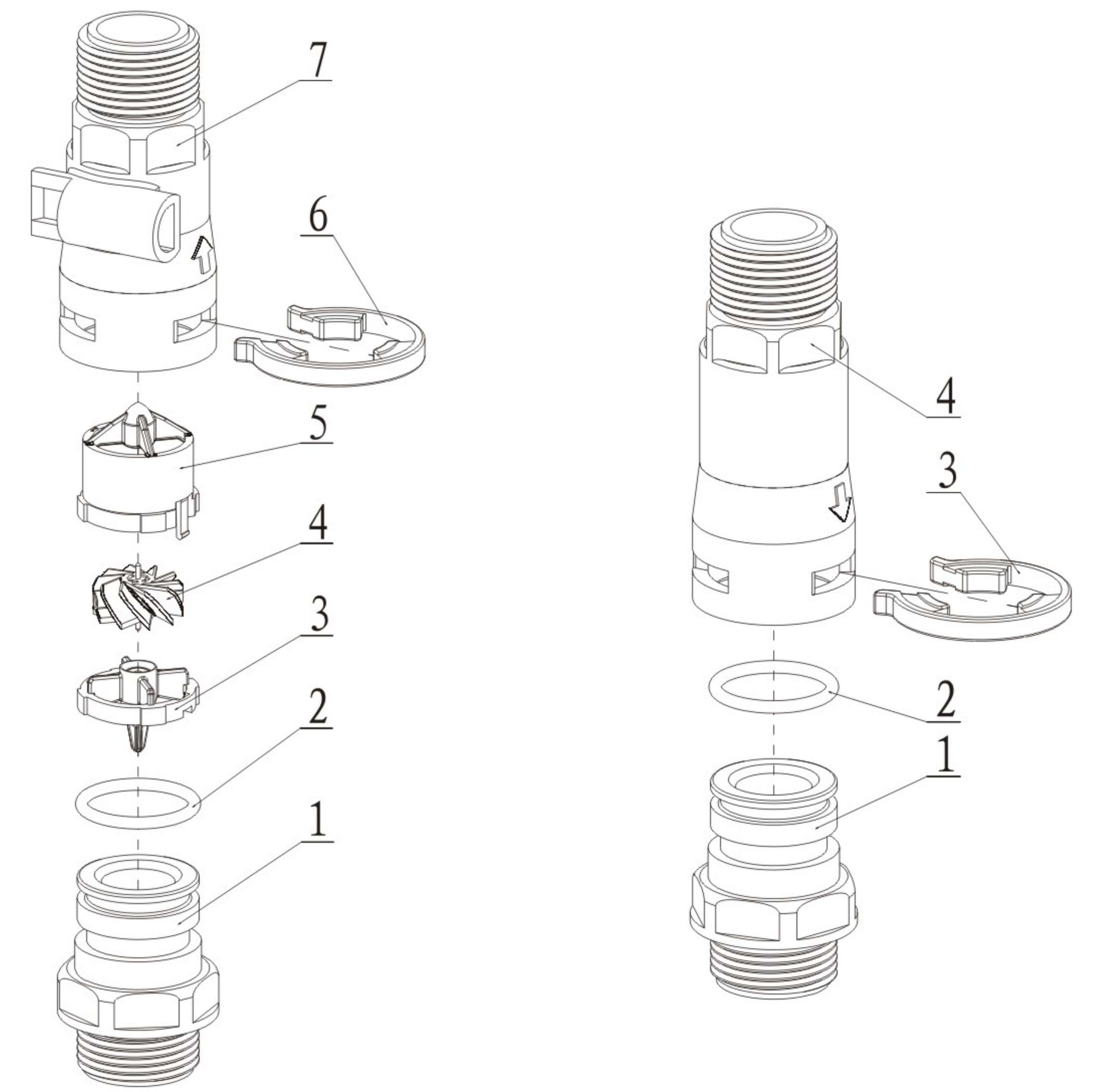
5447020 Flow Meter
