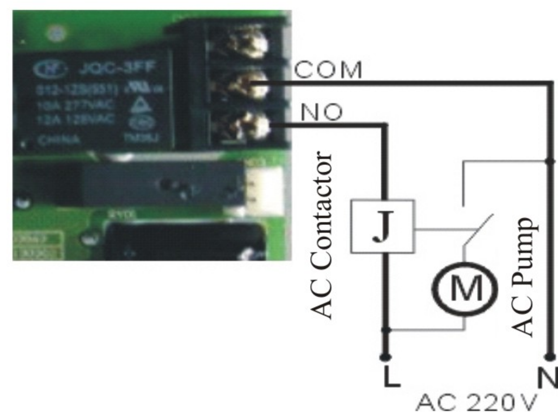
Figure 3-8 Wiring of Booster Pump on Inlet
