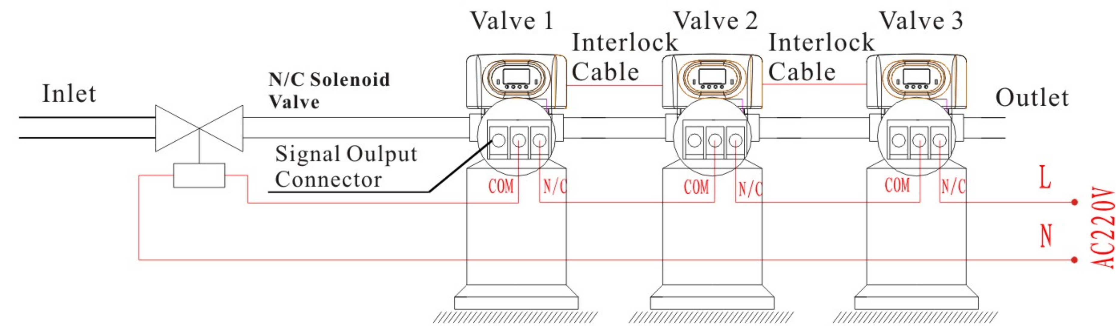
Figure 3-4 Wiring of Solenoid Valve on Inlet
