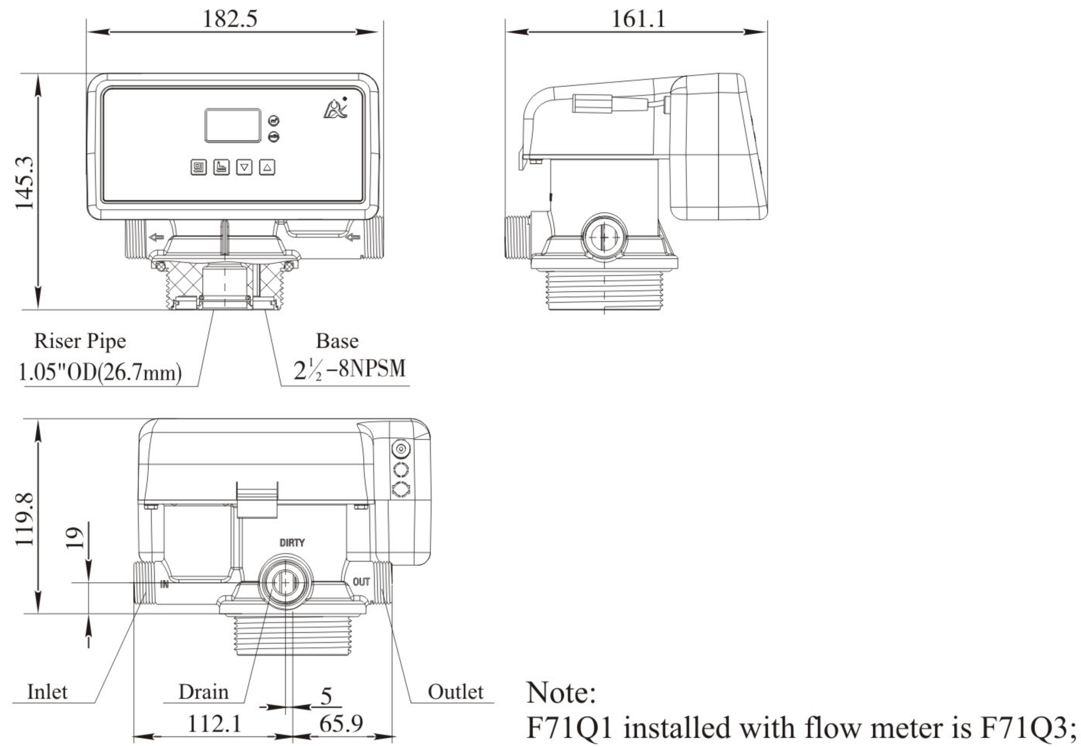
F71Q1 structure chart:
