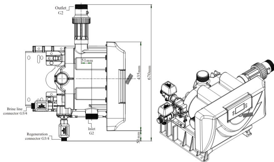
93620 Structural drawing
