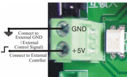
Figure 3-11 Wiring of Remote Input
