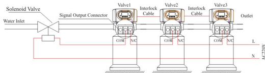
Figure3-4 Wiring of Solenoid Vale in Inlet
