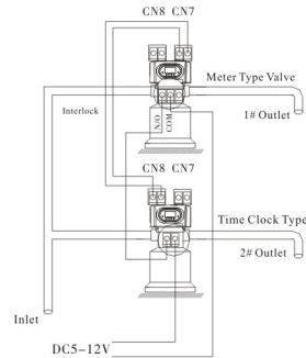
Figure 3-13 Series system
