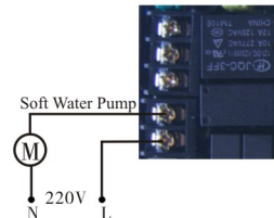
Figure 3-15 Wiring of Soft Water Pump Power Less Than 1KW
