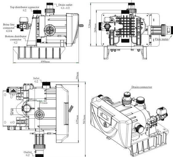
63620 Structural drawing
