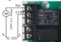
Figure 3-7 Wiring of Booster Pump on Inlet
